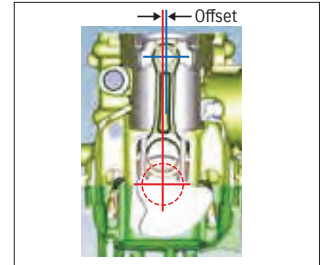
OFFSET CRANKSHAFT
