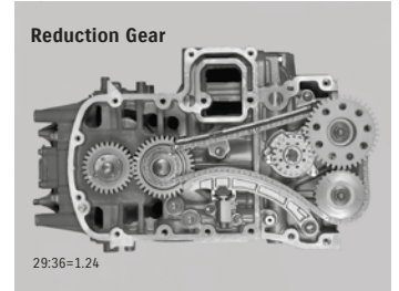
TWO-STAGE GEAR REDUCTION
